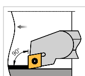
SCFC L/R
