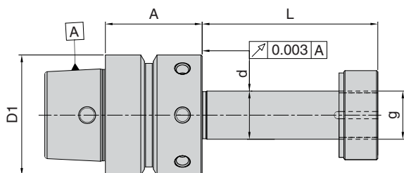
HSK-E50, Ød=20mm
