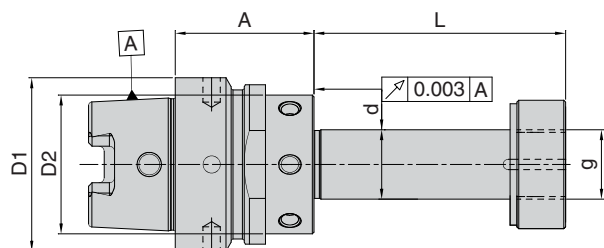
HSK-E50, Ød=20mm
