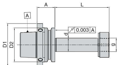
HSK-E50, Ød=20mm
