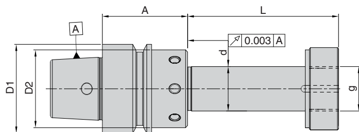
HSK-E40, Ød=20mm
