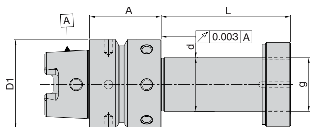
HSK-E50, Ød=31.75mm
